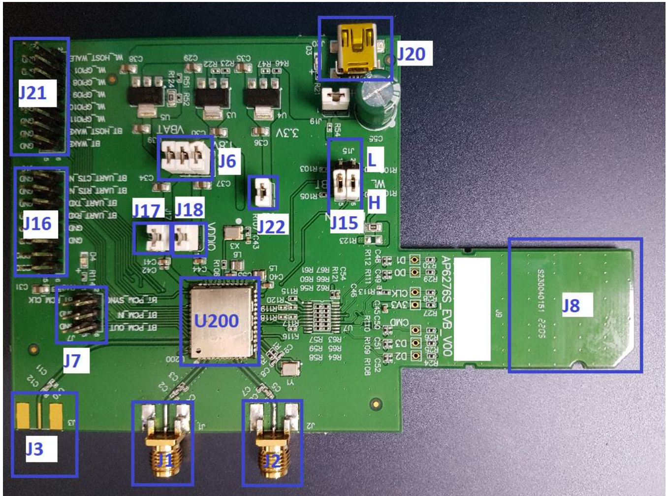
Figure1. Top view of AP6275S EVB
